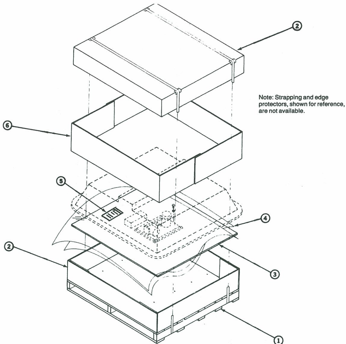
5594000 Repair Carton Assembly (Order By Assembly Number)
