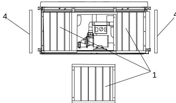
FRONT VIEW (ACCESS VIEW)
