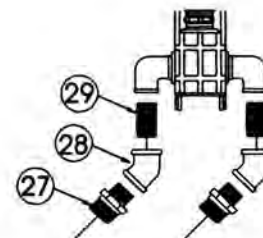
DETAIL 4
