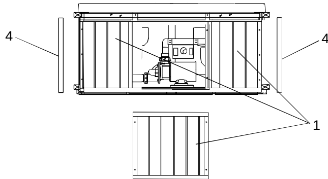
FRONT VIEW (ACCESS VIEW)
