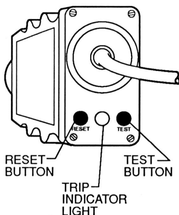
DETAIL OF GFCI
